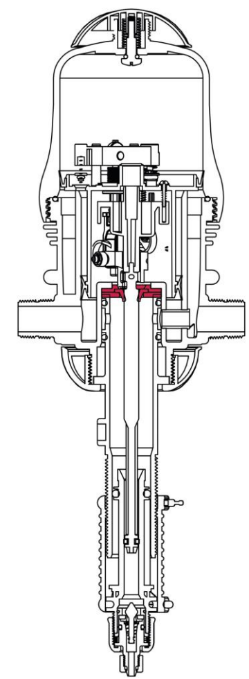
KIT – H Bypass Seal
