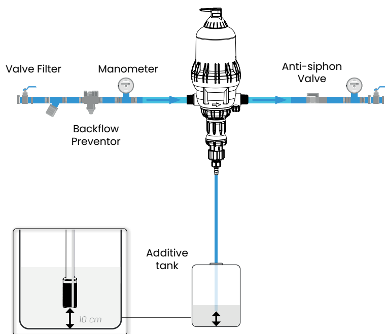
Fig. 2 - Installation illustration
